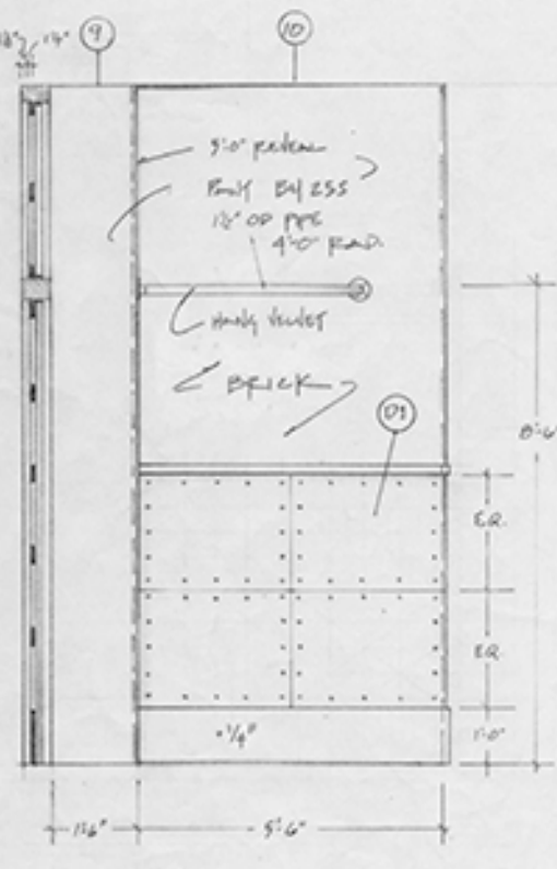
C-C SECTION C-C Scale 1/2" = 1'-0"
