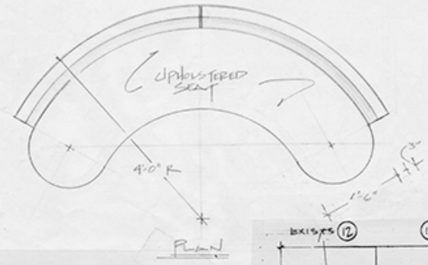
H CURVED BANQUETTE MAKE 2 SCALE 1/2" = 1'-0"
