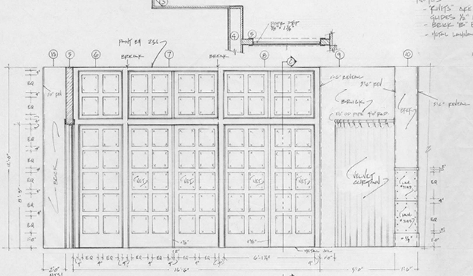
B Upside Window Scale 1/2" = 1'-0"
