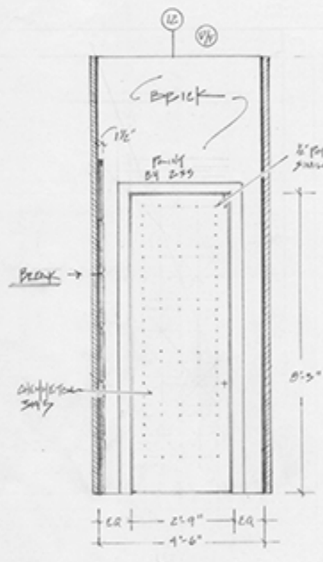
D LSL DOOR SCALE 1/2" = 1'-0"
