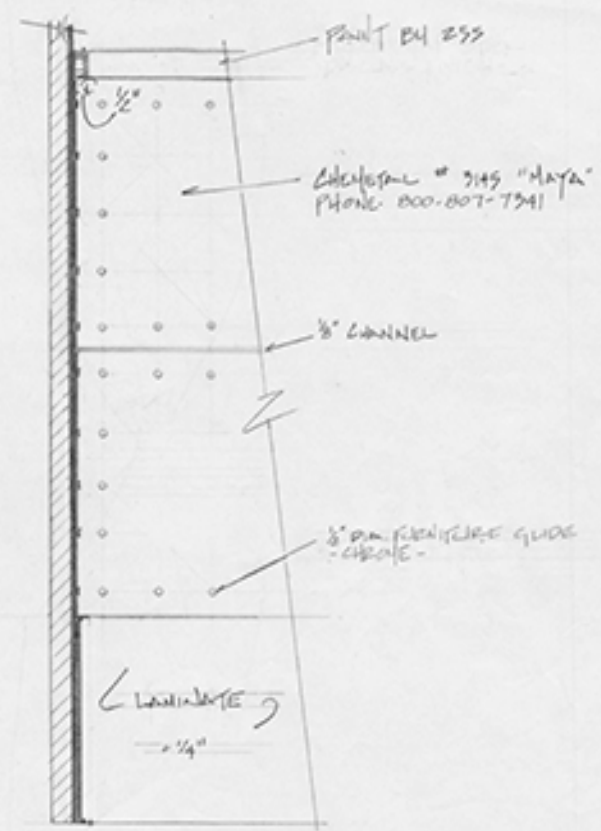
D1 DETAIL #1 Scale 1/2" = 1'-0"
