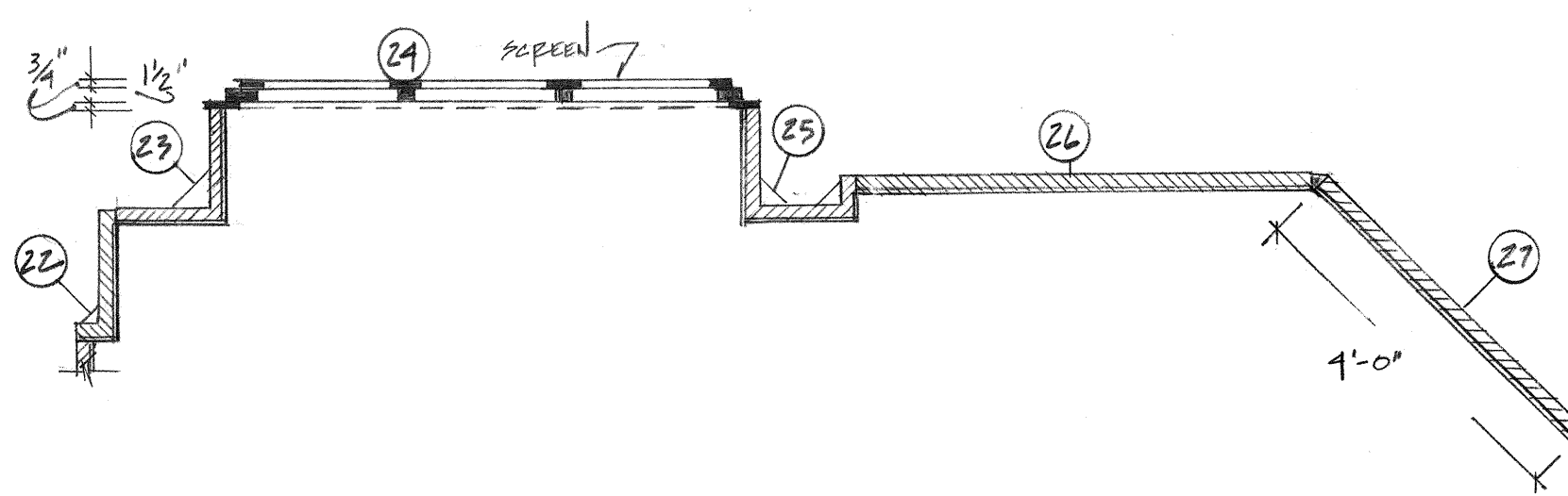
G US HALL WINDOW SCALE 1/2" = 1'-0"
