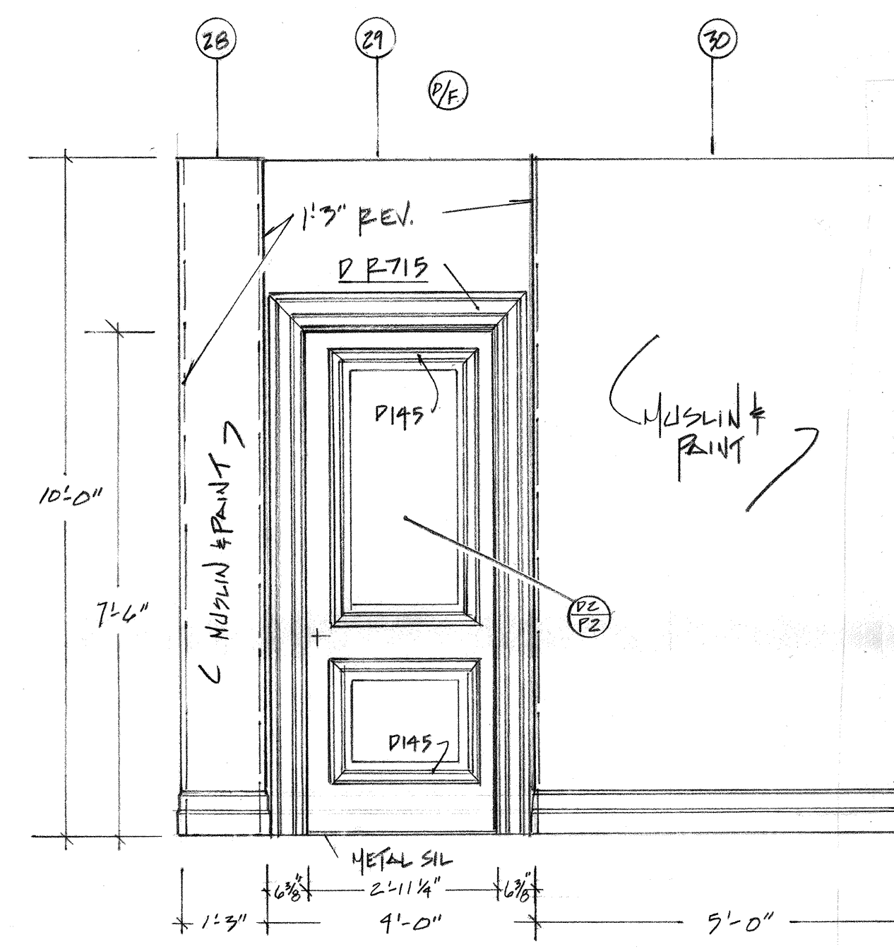
H HALLWAY DOOR S.L. SCALE 1/2" = 1'-0"
