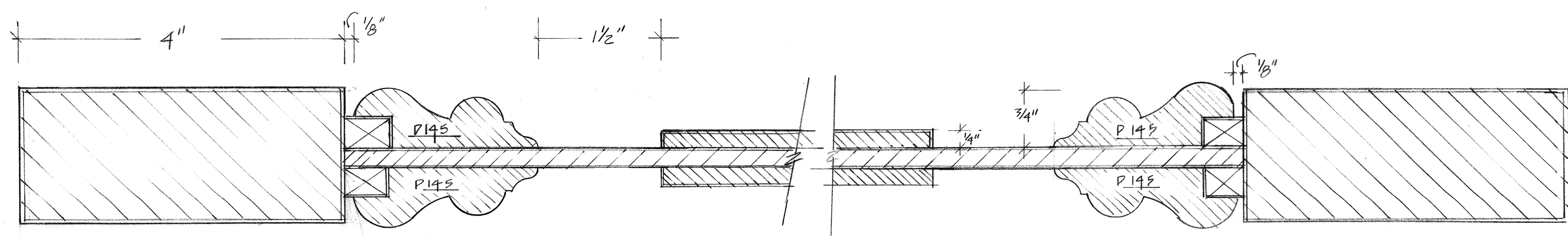
P2 DOOR DETAIL FULL SCALE
