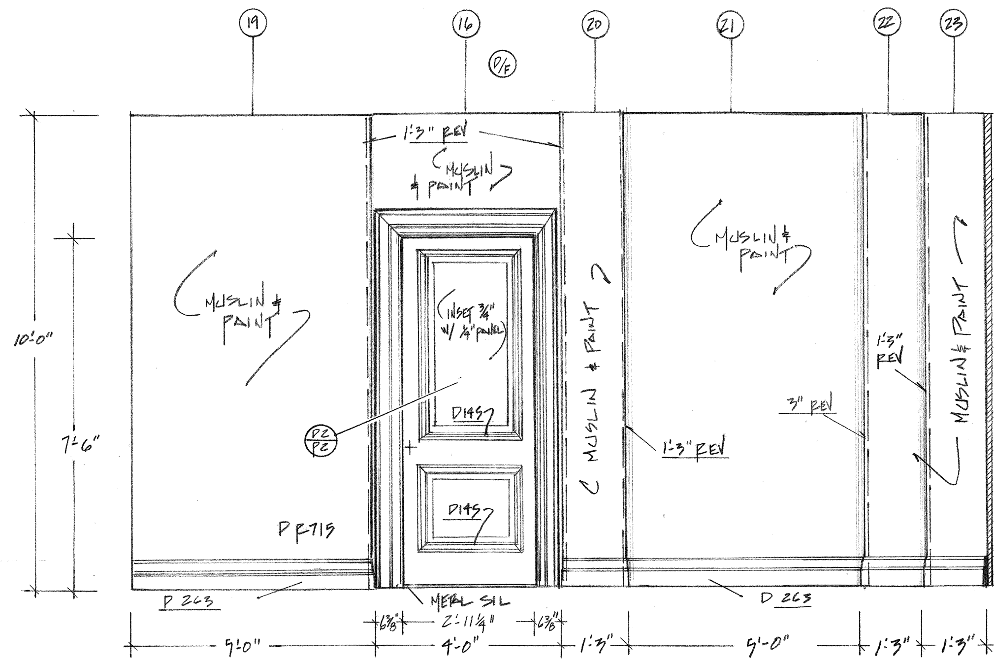
F HALLWAY SR SCALE 1/2" = 1'-0"
