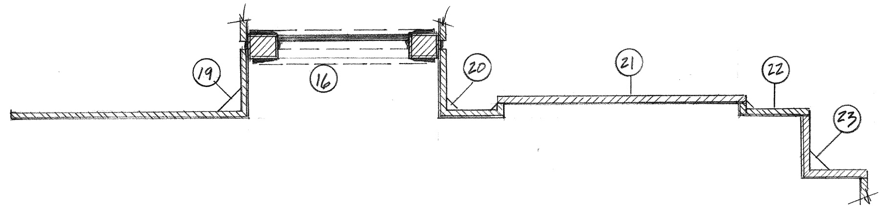
F HALLWAY SR SCALE 1/2" = 1'-0"
