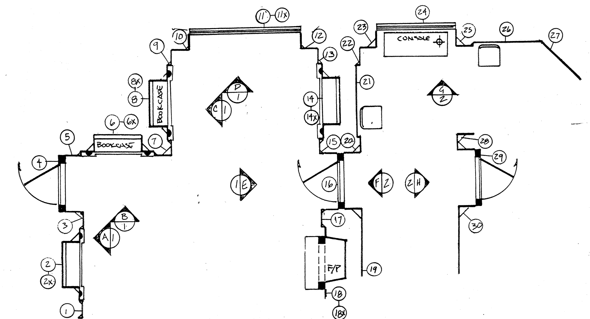
CHANDLER LIBRARY SCALE 1/4" = 1'-0"
