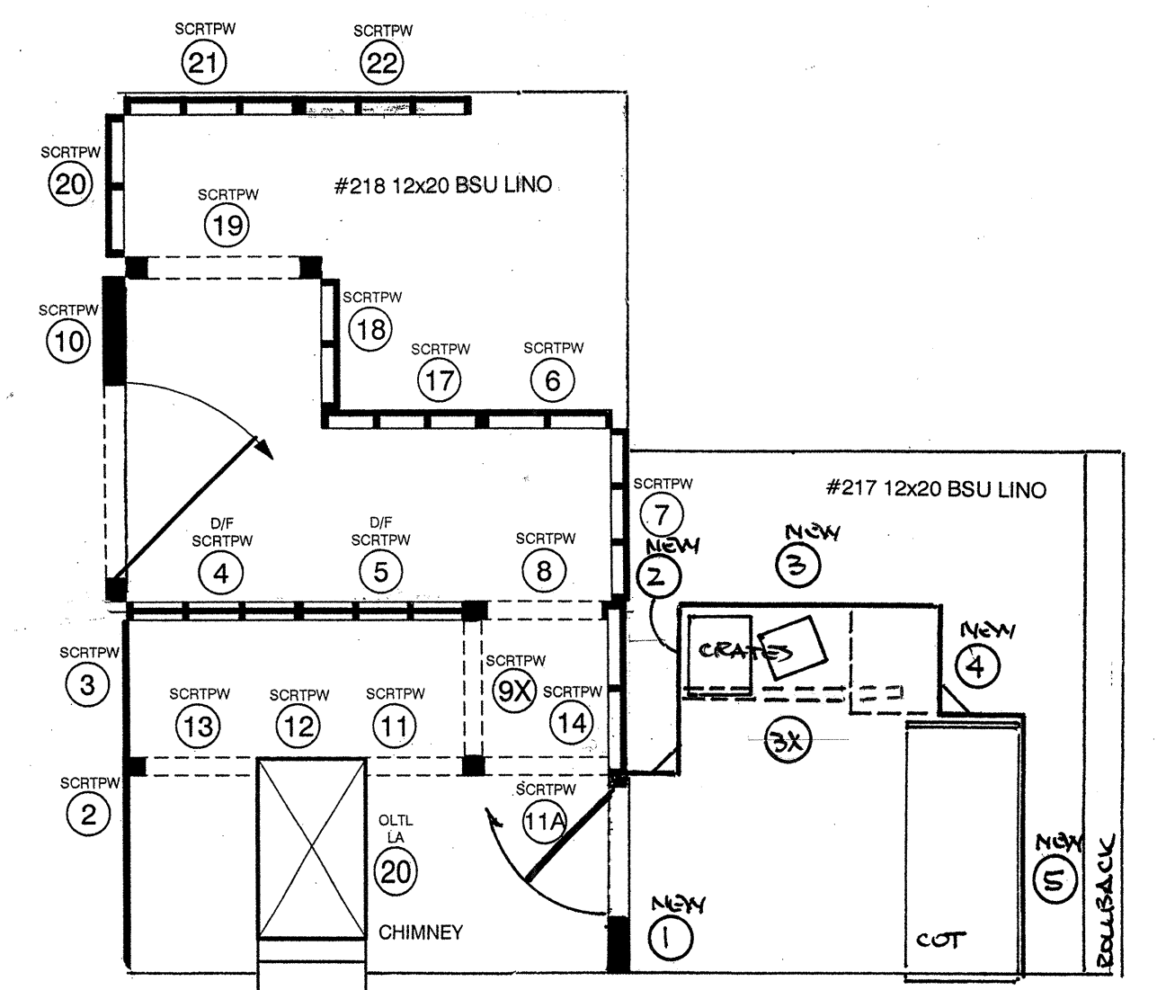
CHANDLER BDRM & OLT L LORD ATTIC AS: CHANDLER SECRET PASSAGEWAY & SECRET ROOM SCALE: 1/4" = 1'-0"
