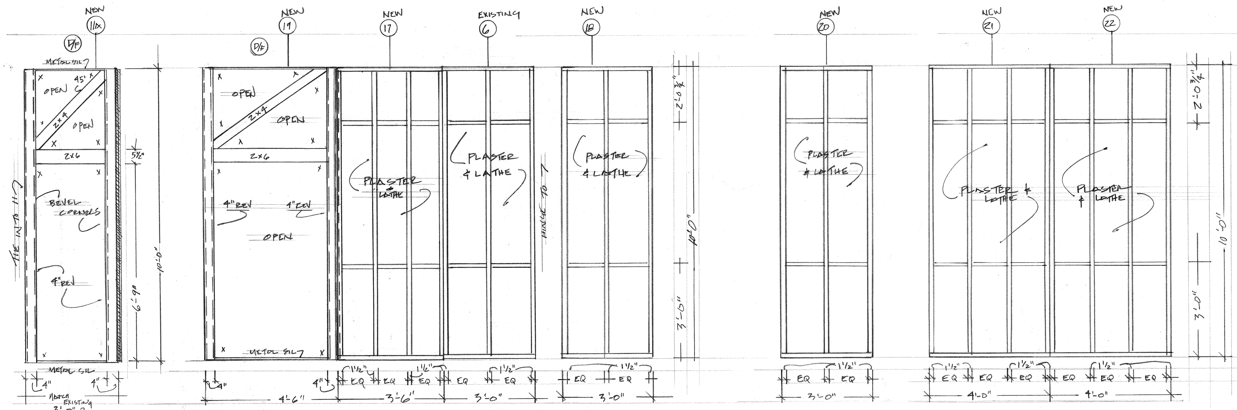
NEW SURET PASSAGE WINGS 12-6-07 SCALE 1/2" = 1'-0"
