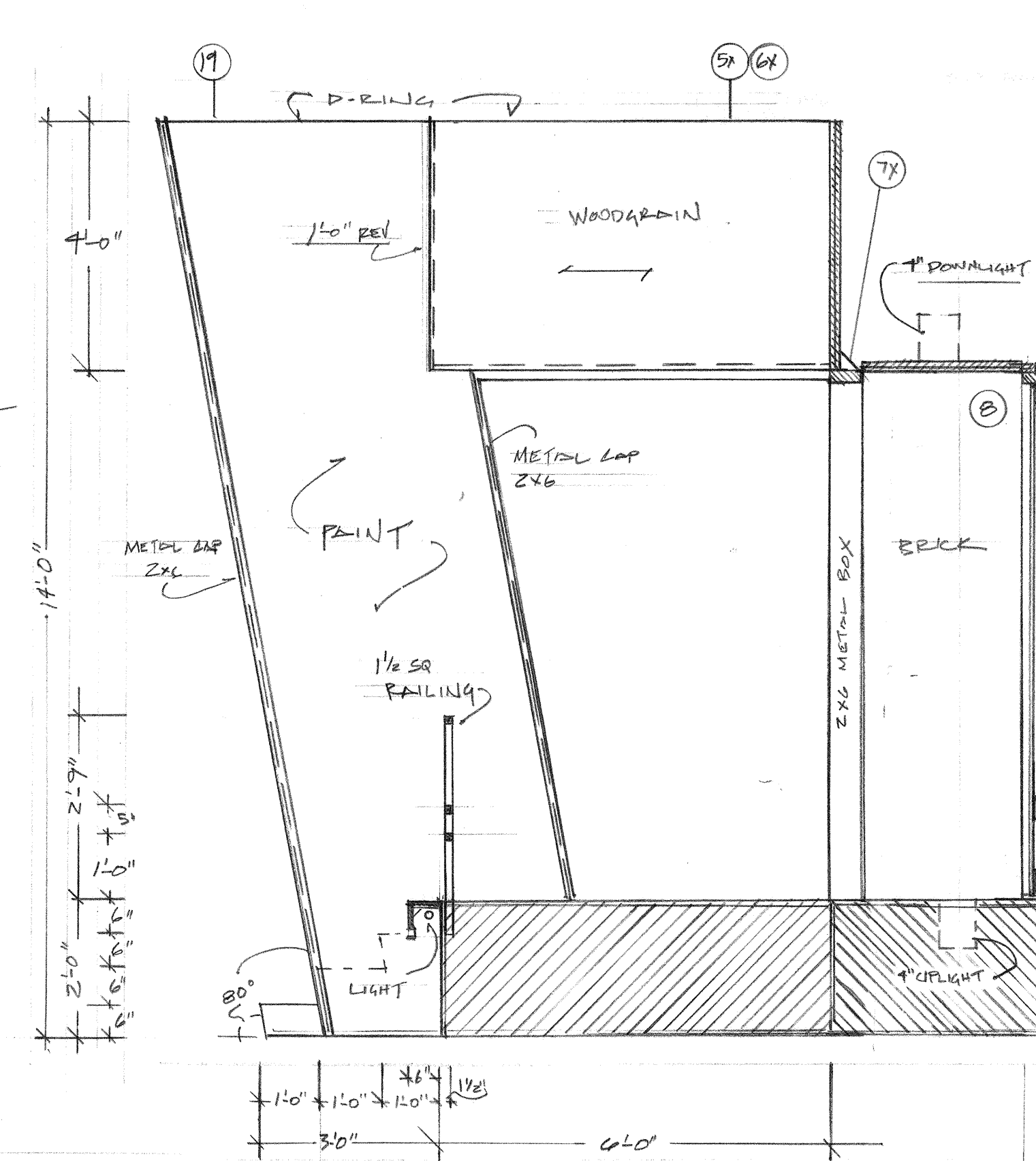
A.A. SECTION A-A SCALE 1/2"=1'-0"
