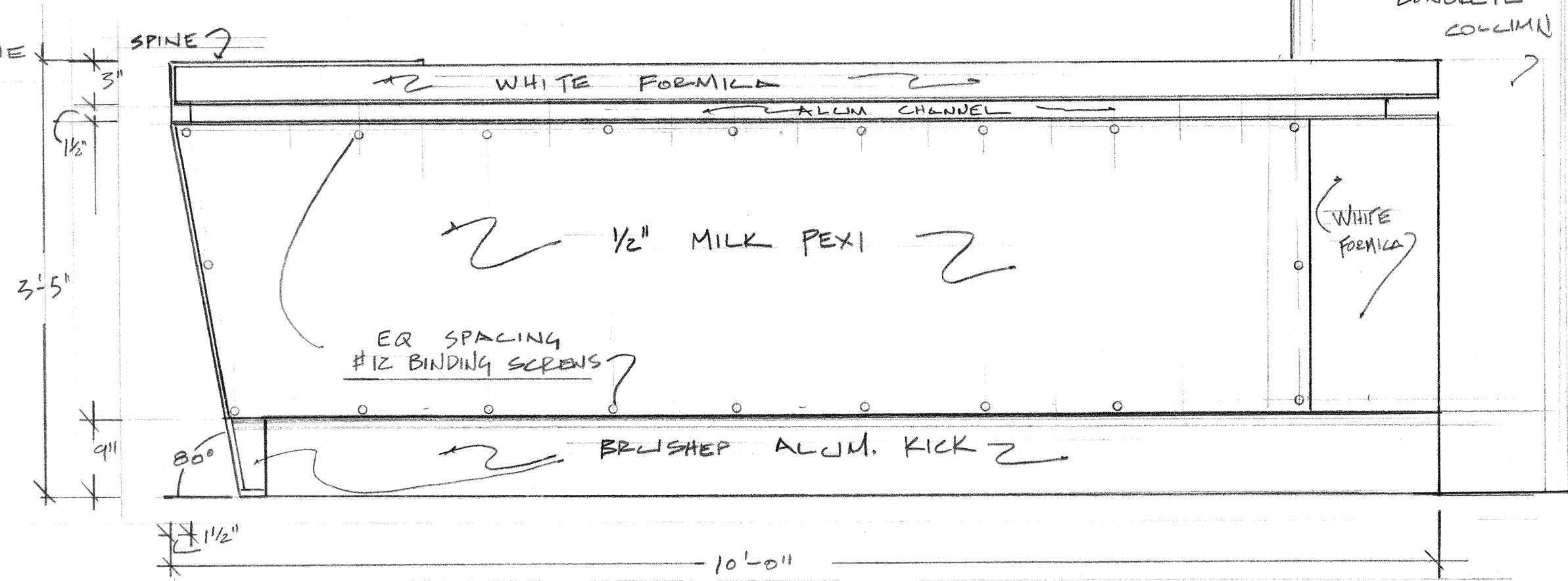
F U.S. BAR FACE SCALE 1"=1'-0"
