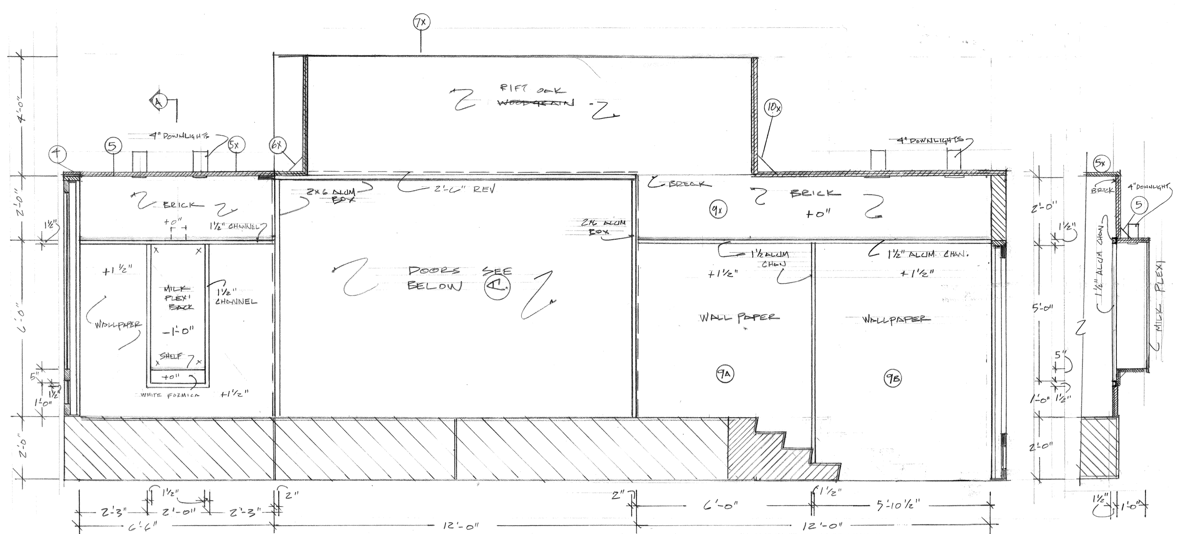
A-A SECTION A-A SCALE 1/2"=1'-0"
