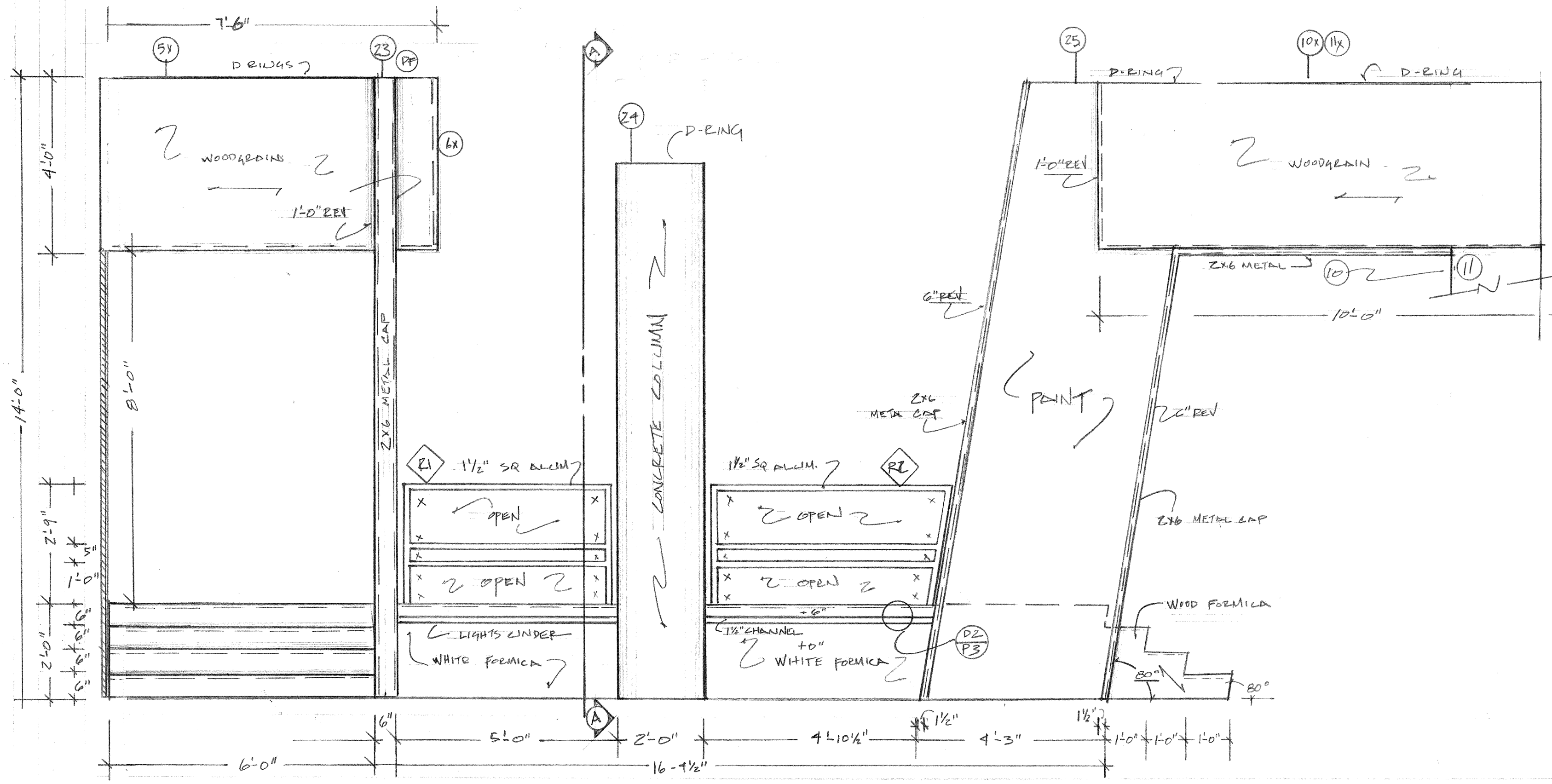
H PLATFORM & FACING SCALE 1/2"=1'-0"
