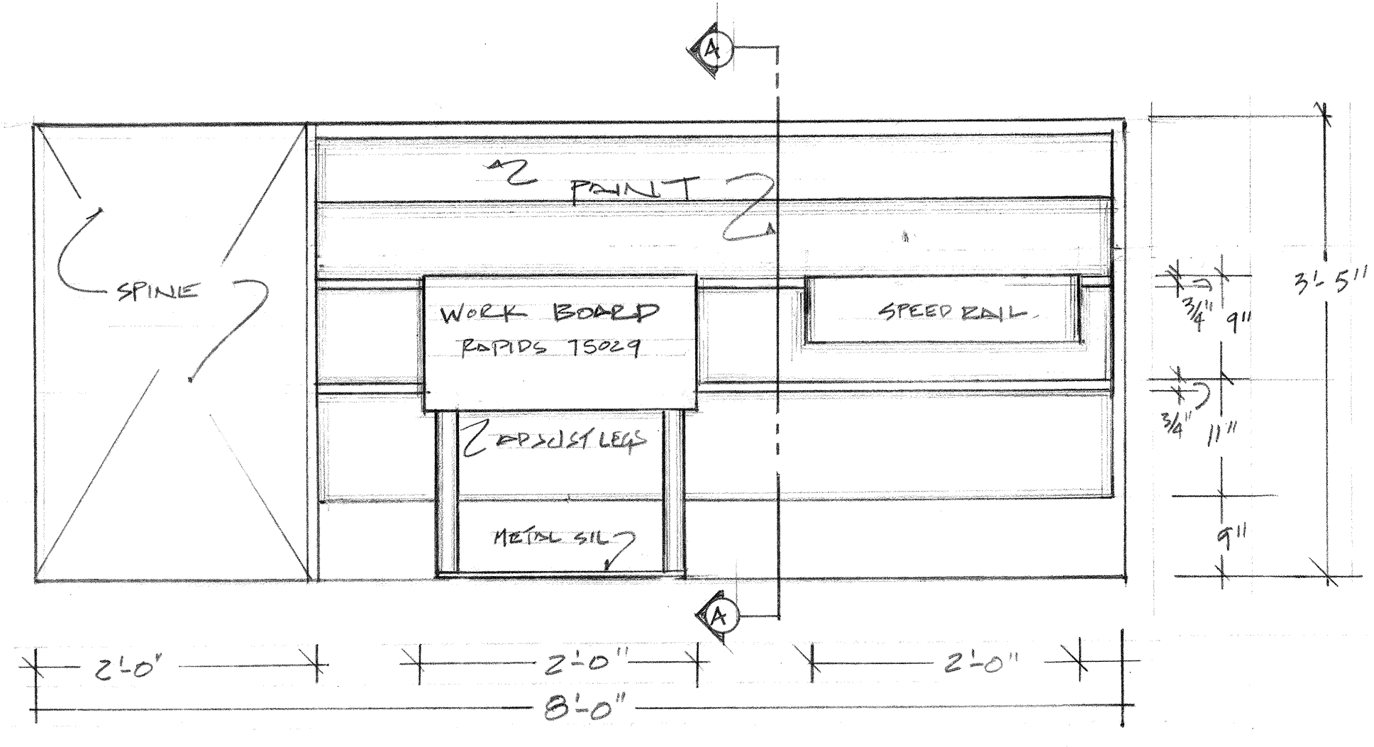
D SL BAR INSIDE SCALE 1"=1'-0"
