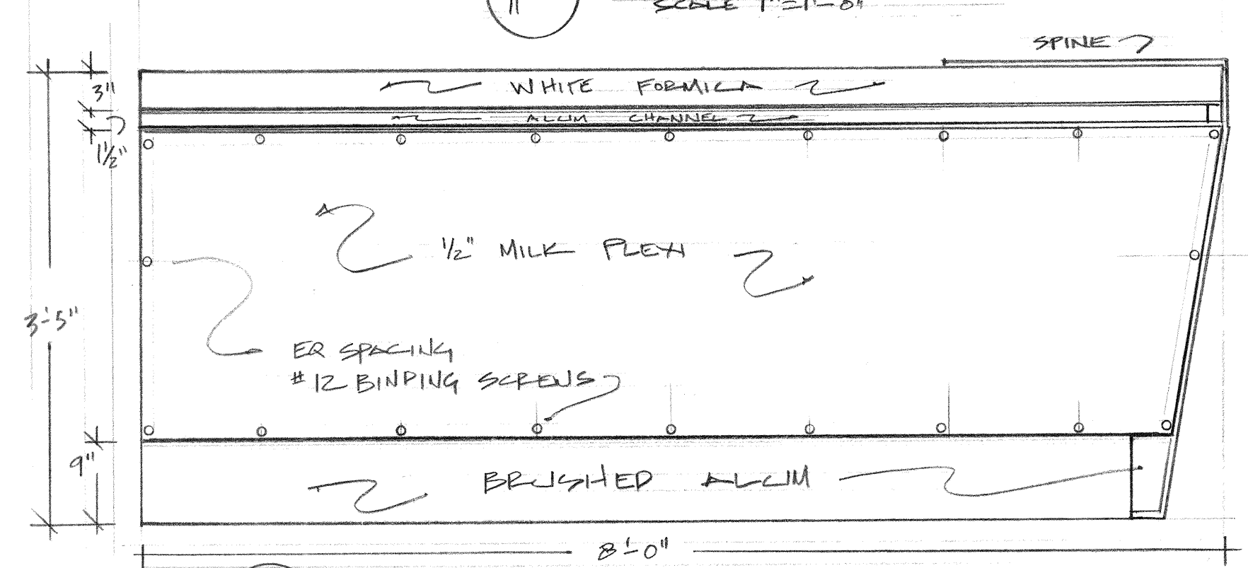
G SL BAR FACE SCALE 1"=1'-0"
