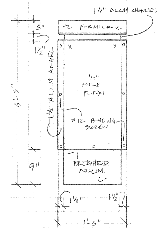
BAR TABLE MAKE 3 SCALE 1/2"=1'-0"
