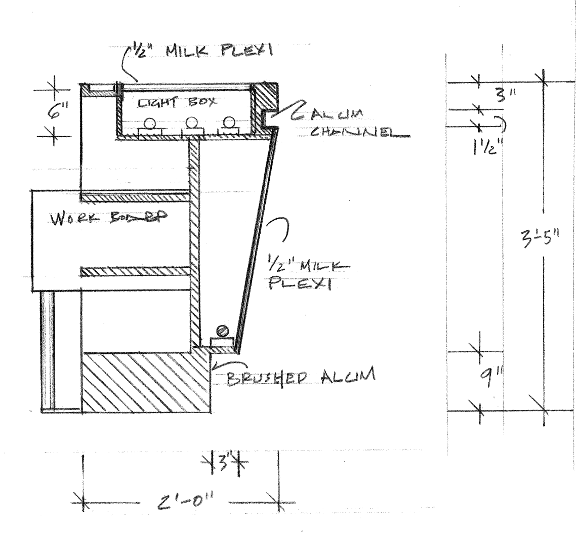
A-A SECTION A-A SCALE 1"=1'-0"
