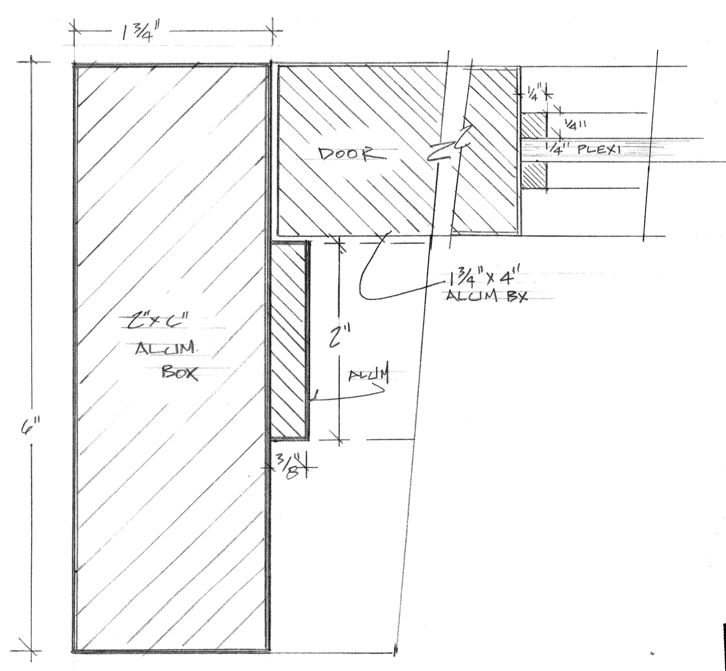
D1 DOOR DETAIL FULL SCALE
