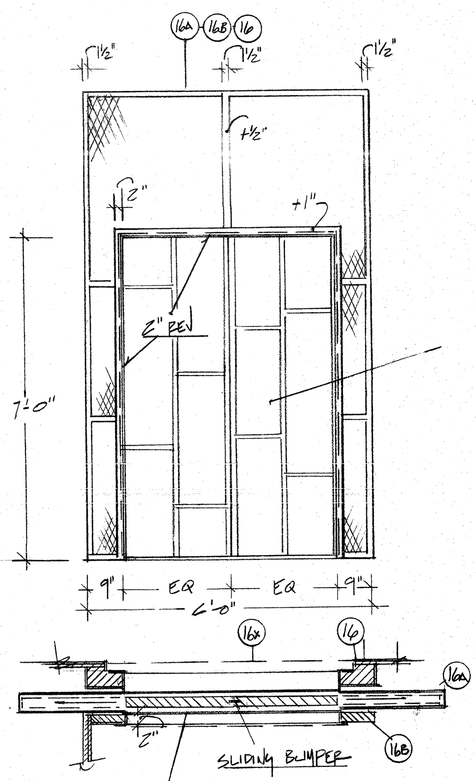
C ELEVATOR DOORS & CAB SCALE 1/2" = 1'-0"
