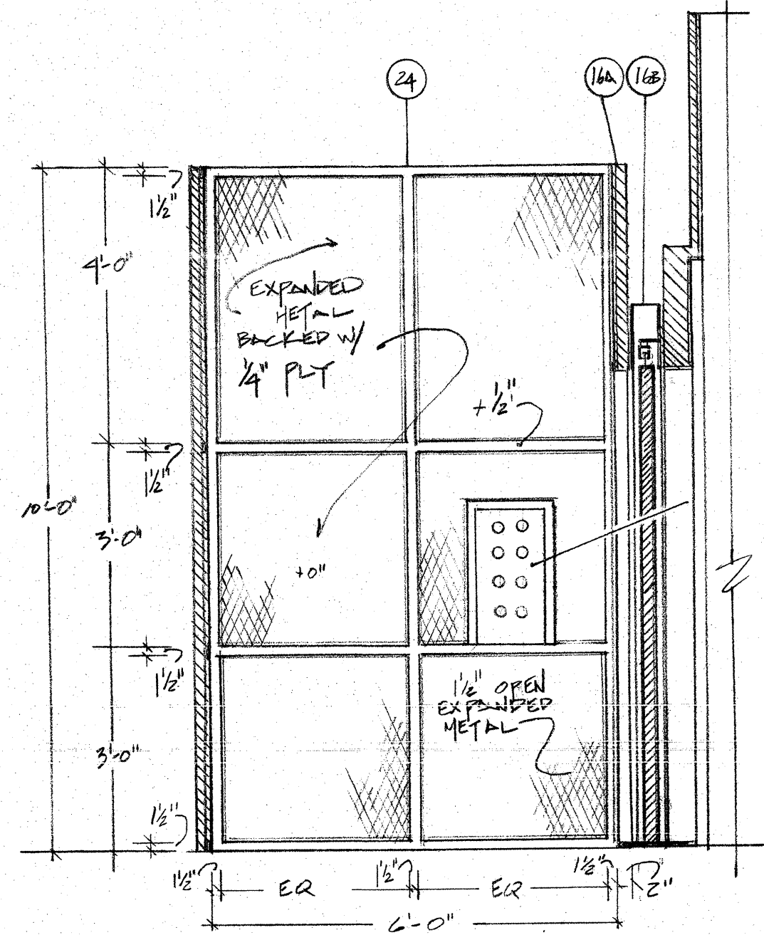
B ELEVATOR CAB LS SCALE 1/2" = 1'-0"
