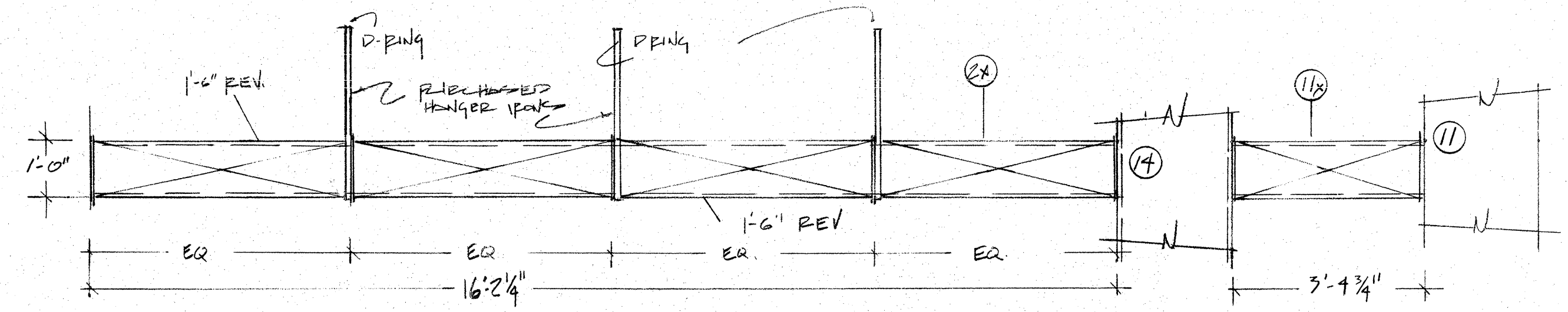
E. ELEVATOR FACE SCALE 1/2" = 1'-0"
