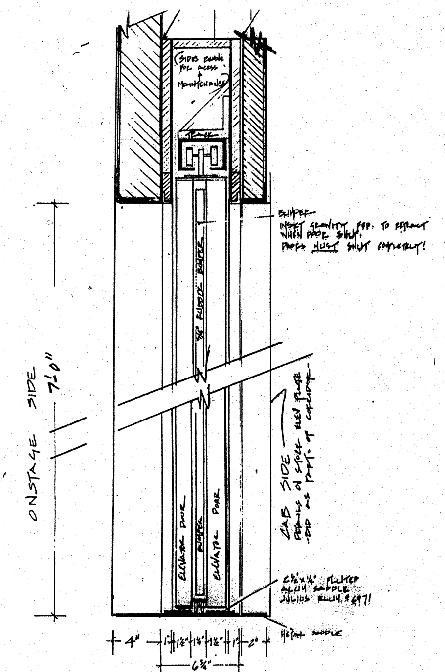
E ELEVATOR DETAIL SCALE 1/2" = 1'-0"
