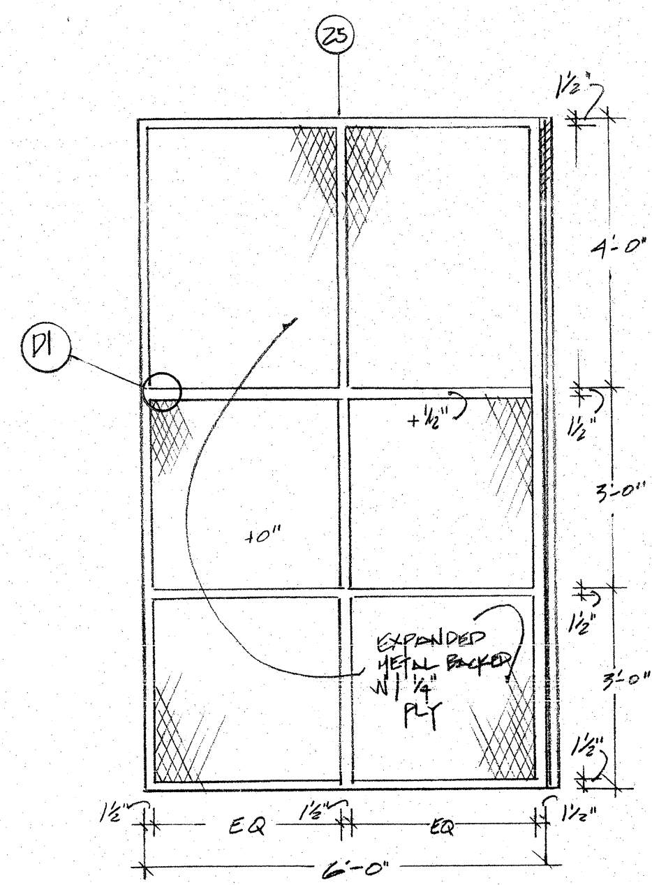
A ELEVATOR SP SCALE 1/2" = 1'-0"
