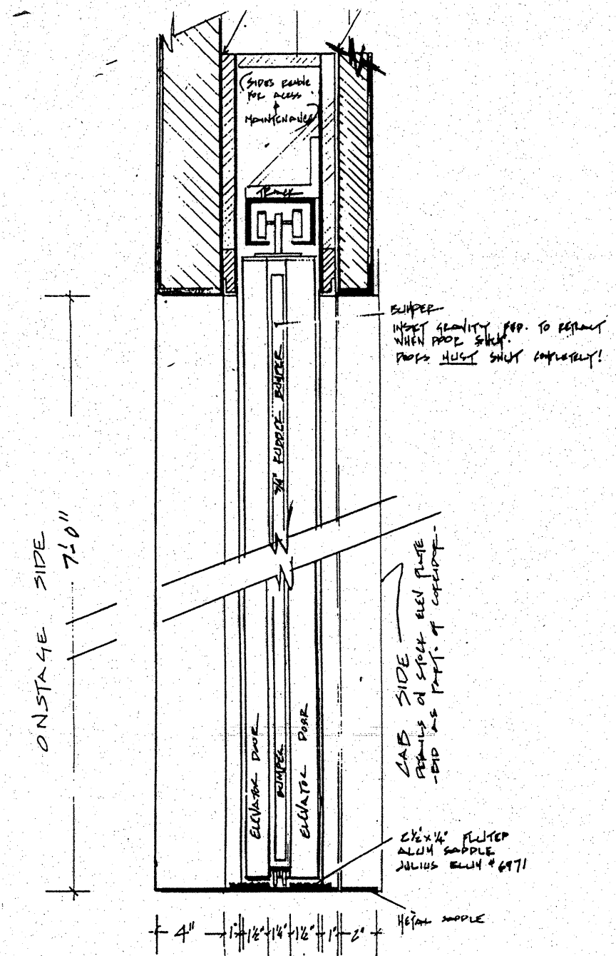
ELEVATOR DETAIL SCALE 1/2" = 1'-0"
