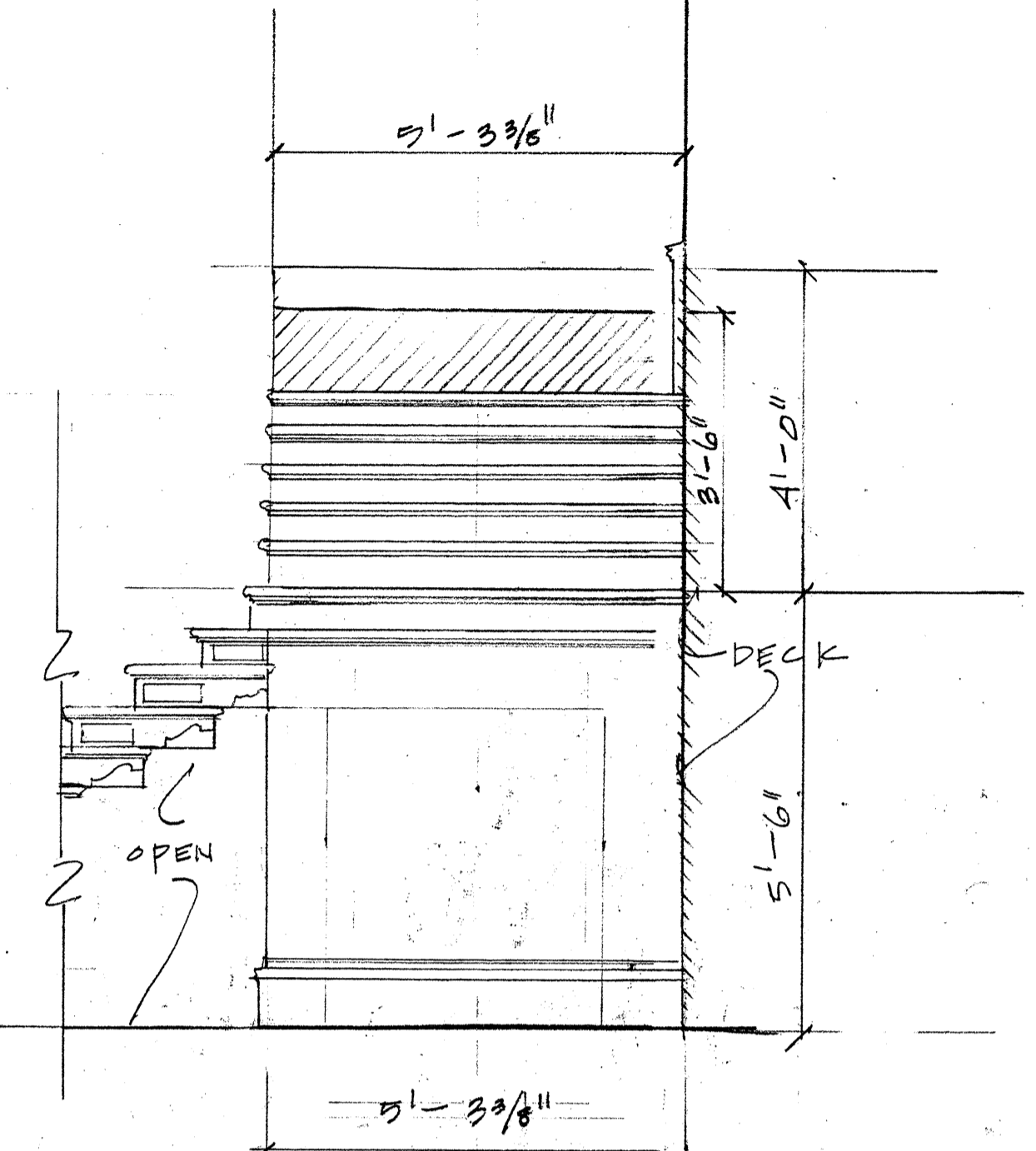
(C) SIDE VIEW STAIRS R.H. UNDER STAIR PLATFORM C
