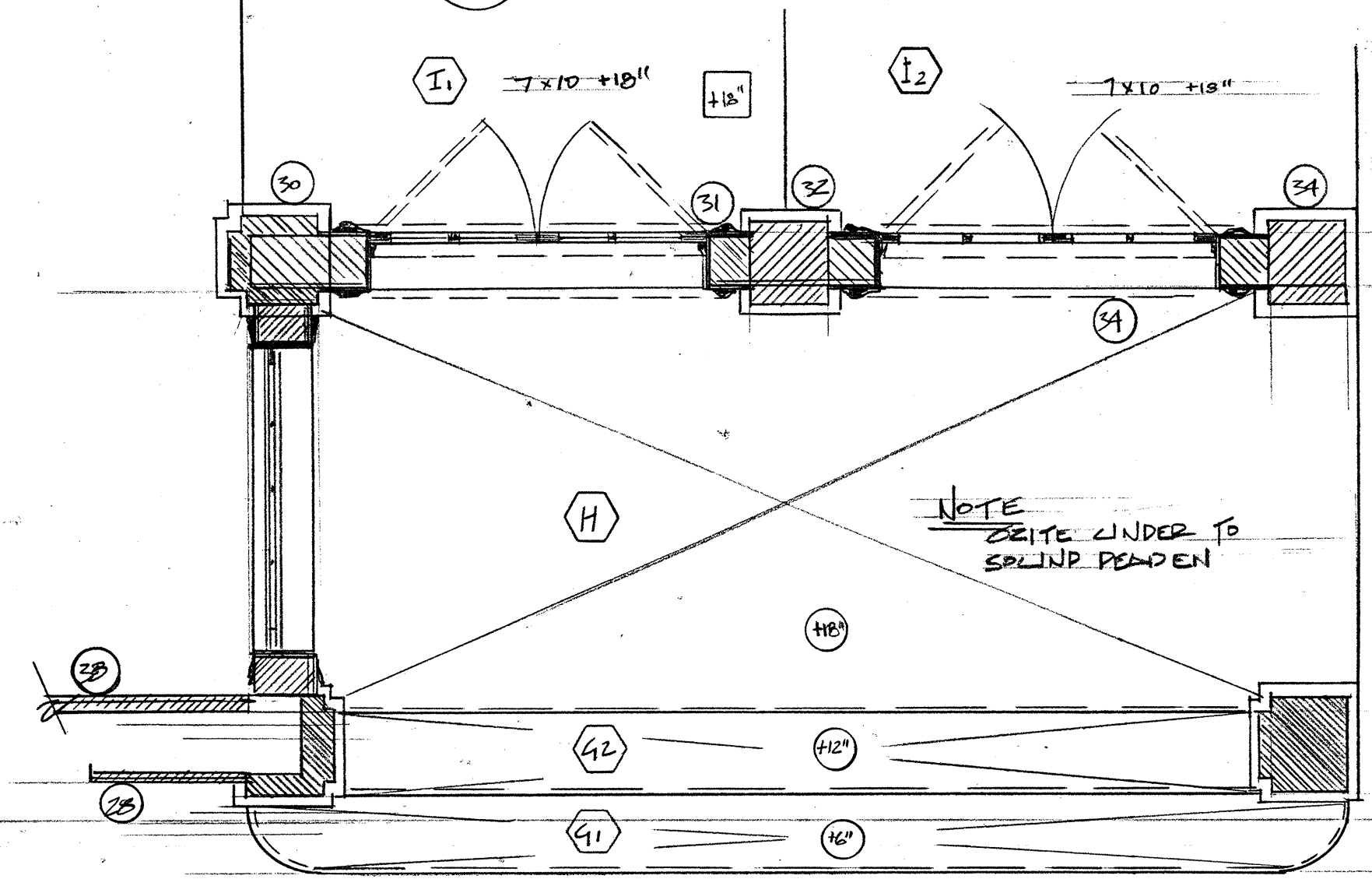
J DOOR ARCHWAY SCALE 1/2" = 1'-0"
