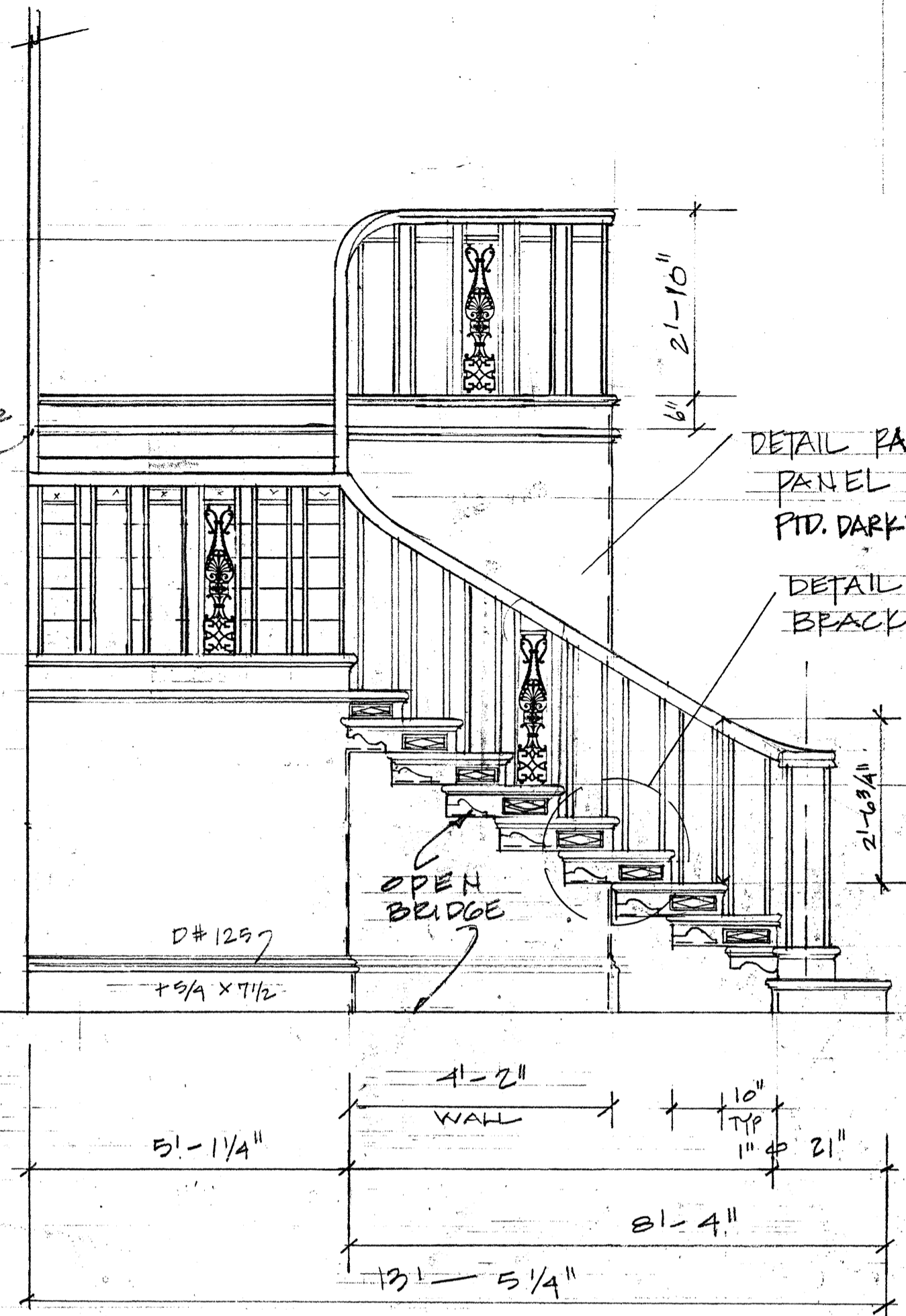
(B) SIDE VIEW STAIRS L.H.
