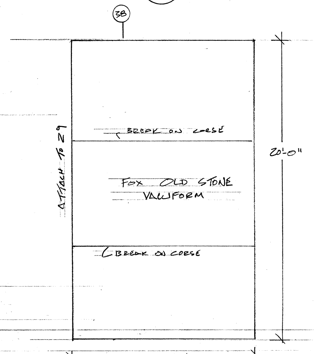
M BRICK WALL SCALE 1/2" = 1'-0"
