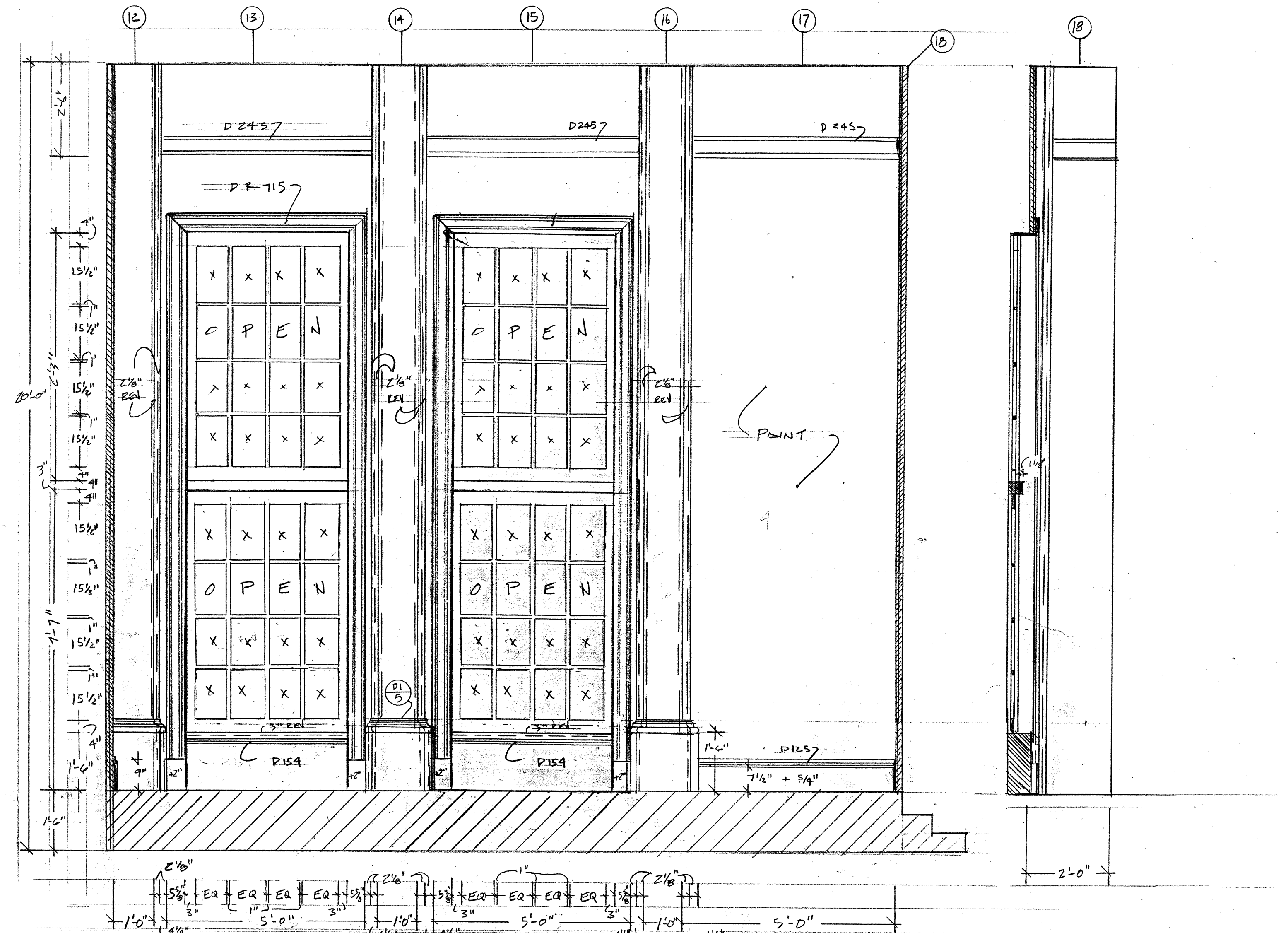
I S WINDOWS SCALE 1/2"=1'-0"
