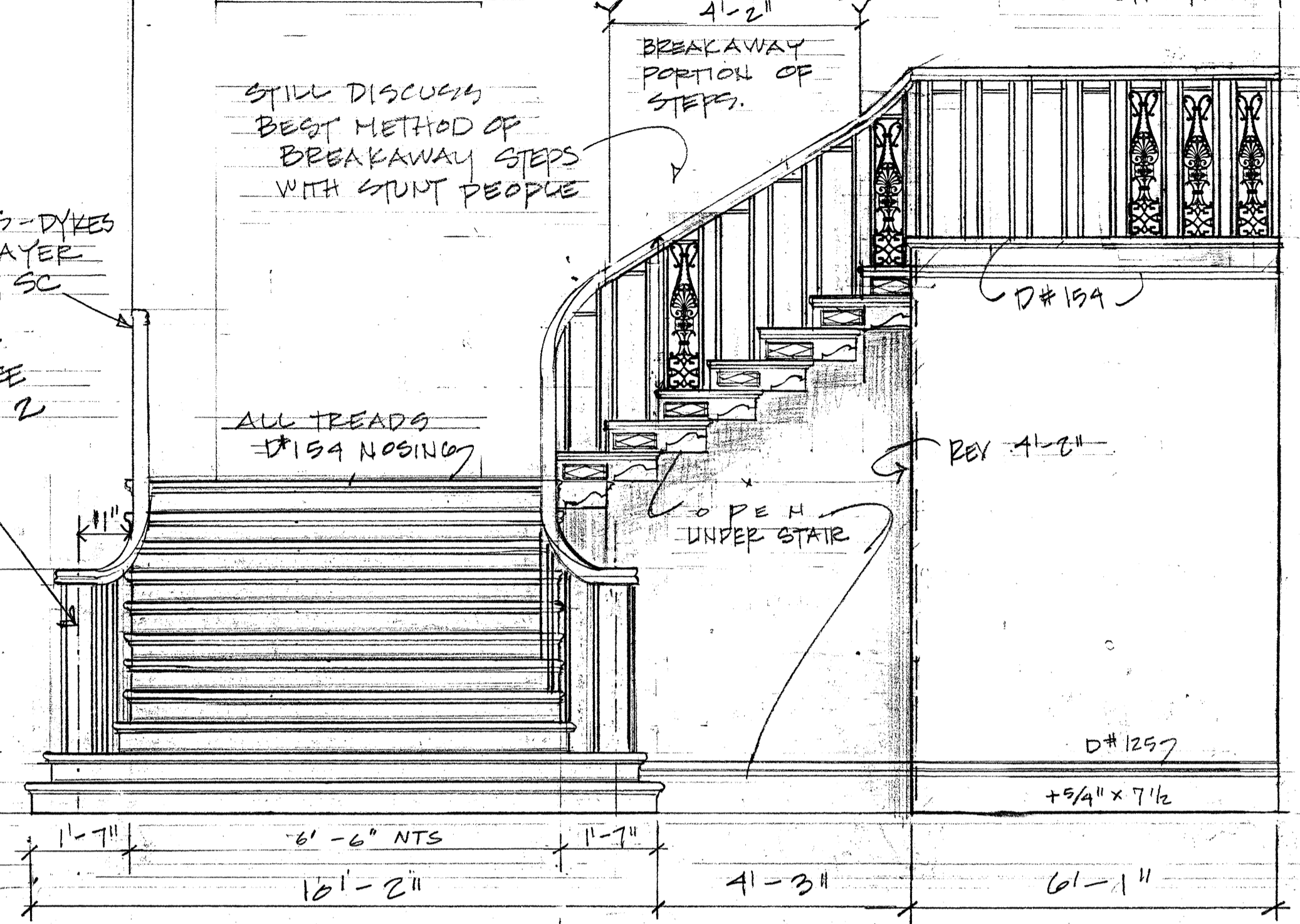
(A) STAIR FACE
