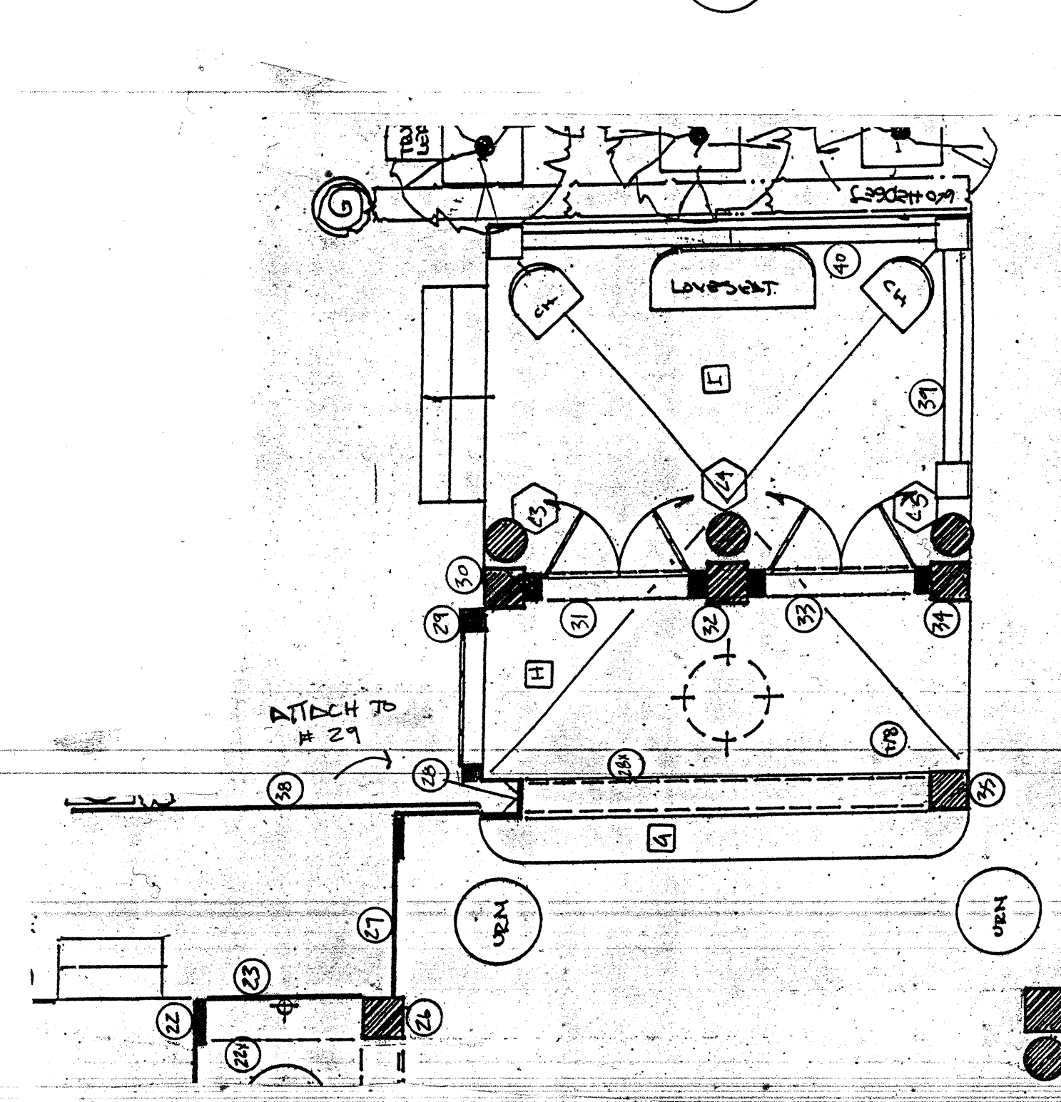
K TERRACE DOORS SCALE 1/2" = 1'-0"
