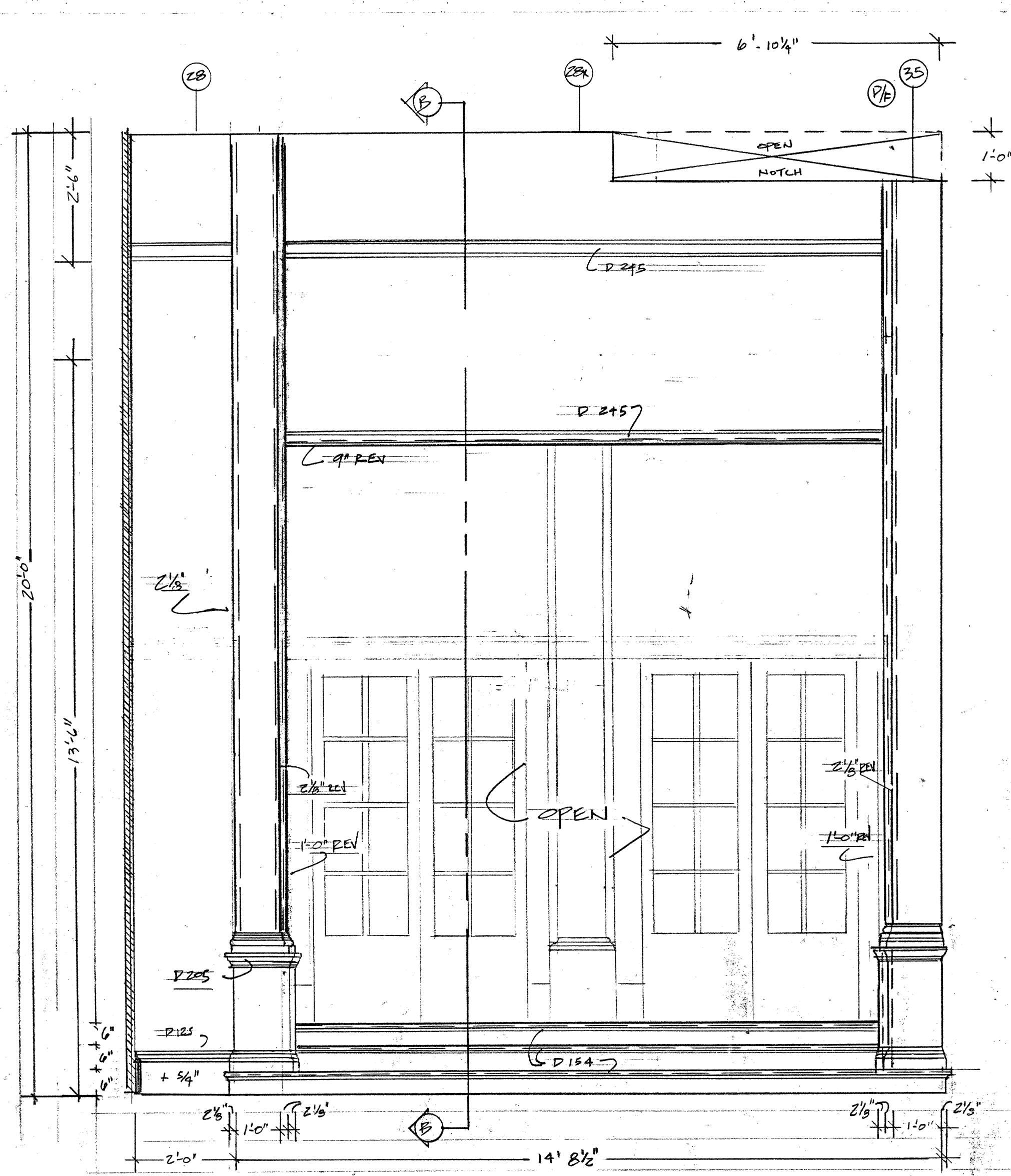
J DOOR ARCHWAY SCALE 1/2" = 1'-0"
