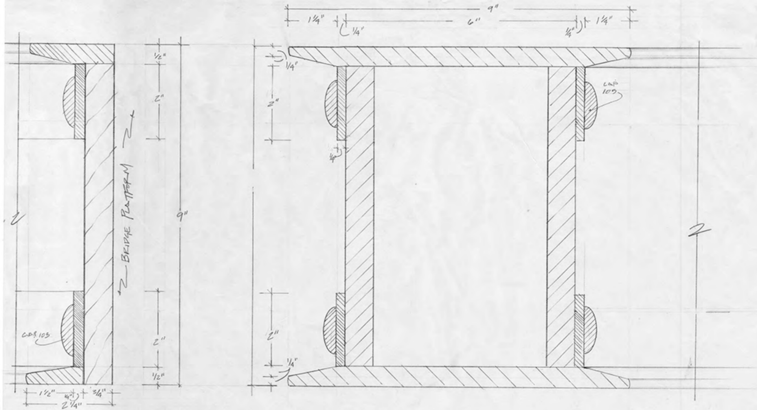
P1 Platform Facing Detail FULL SCALE
