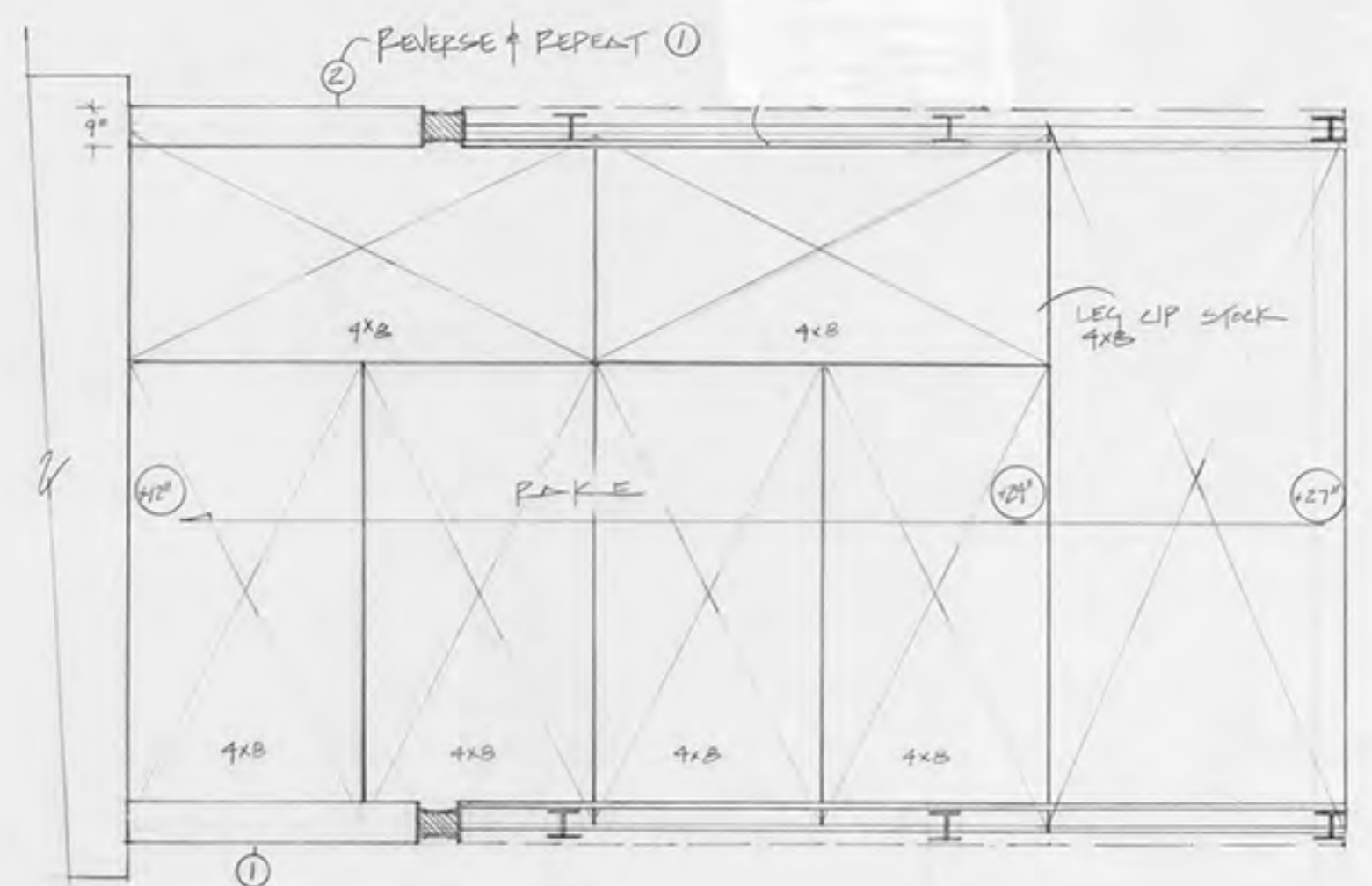
PLAN
