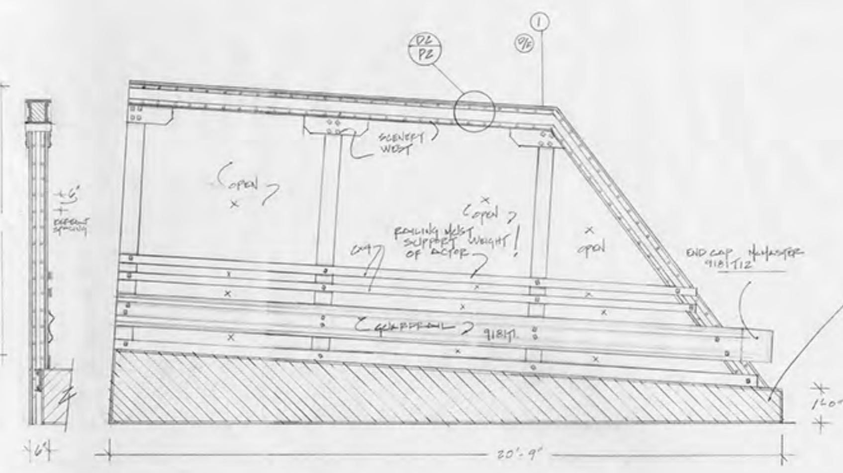
B PS BRIDGE INSIDE SCALE 1/2" = 1'-0"
