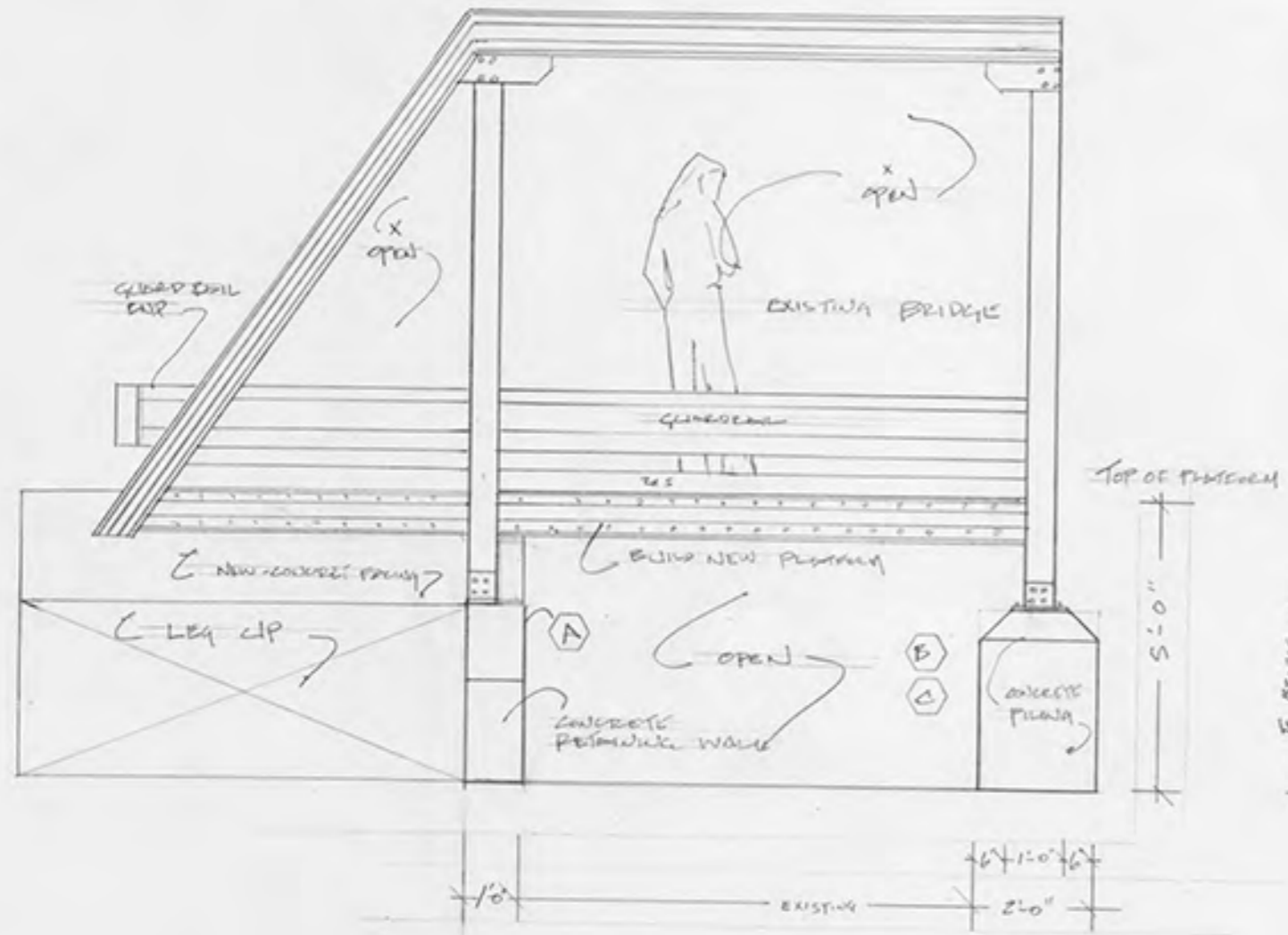
BRIDGE SIDE VIEW SCALE 1/2"=1'-0"
