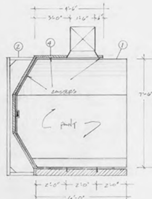
C COMPACTOR WALL SCALE 1/2" = 1'-0" - COMPACTOR WALL CASTED & MOVED BY STAGEHANDS
