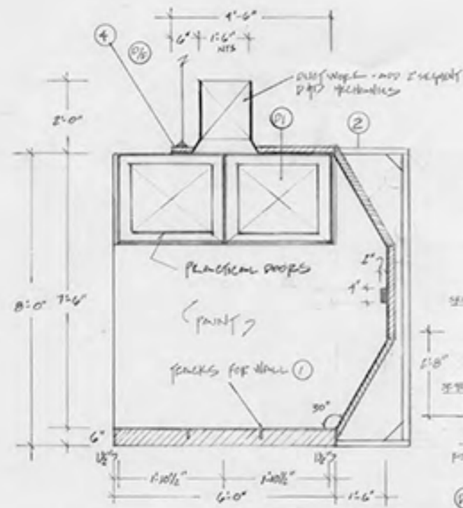
A ENTRANCE SCALE 1/2" = 1'-0"
