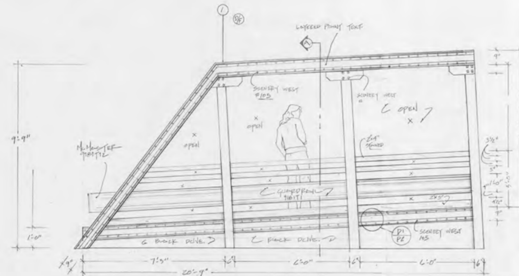
A VS BRIDGE FRONT SCALE 1/2" = 1'-0"
