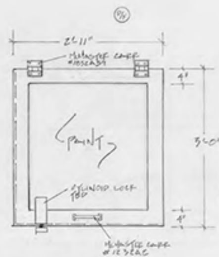
P1 DOOR DETAIL SCALE 1" = 1'-0"
