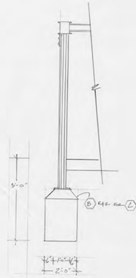
PILING SCALE 1/2"=1'-0"
