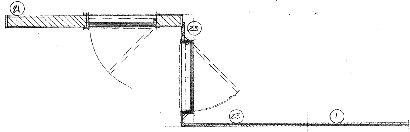
A SR HALLWAY SCALE 1/2"=1'-0"
