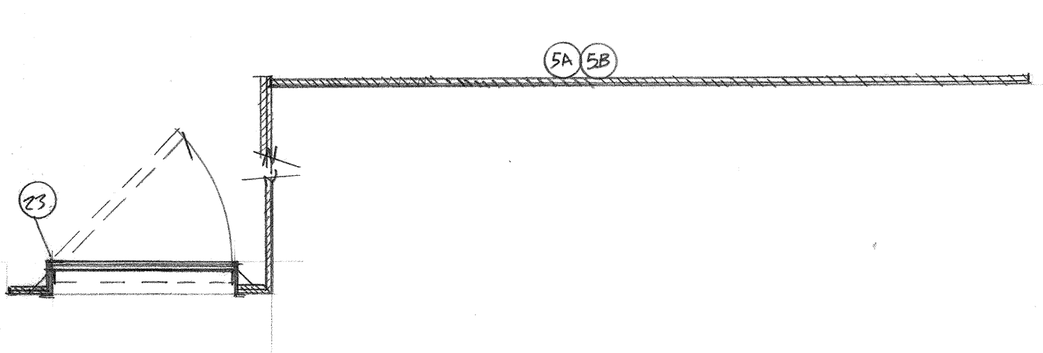
B JAIL HALLWAY SCALE 1/2"=1'-0"
