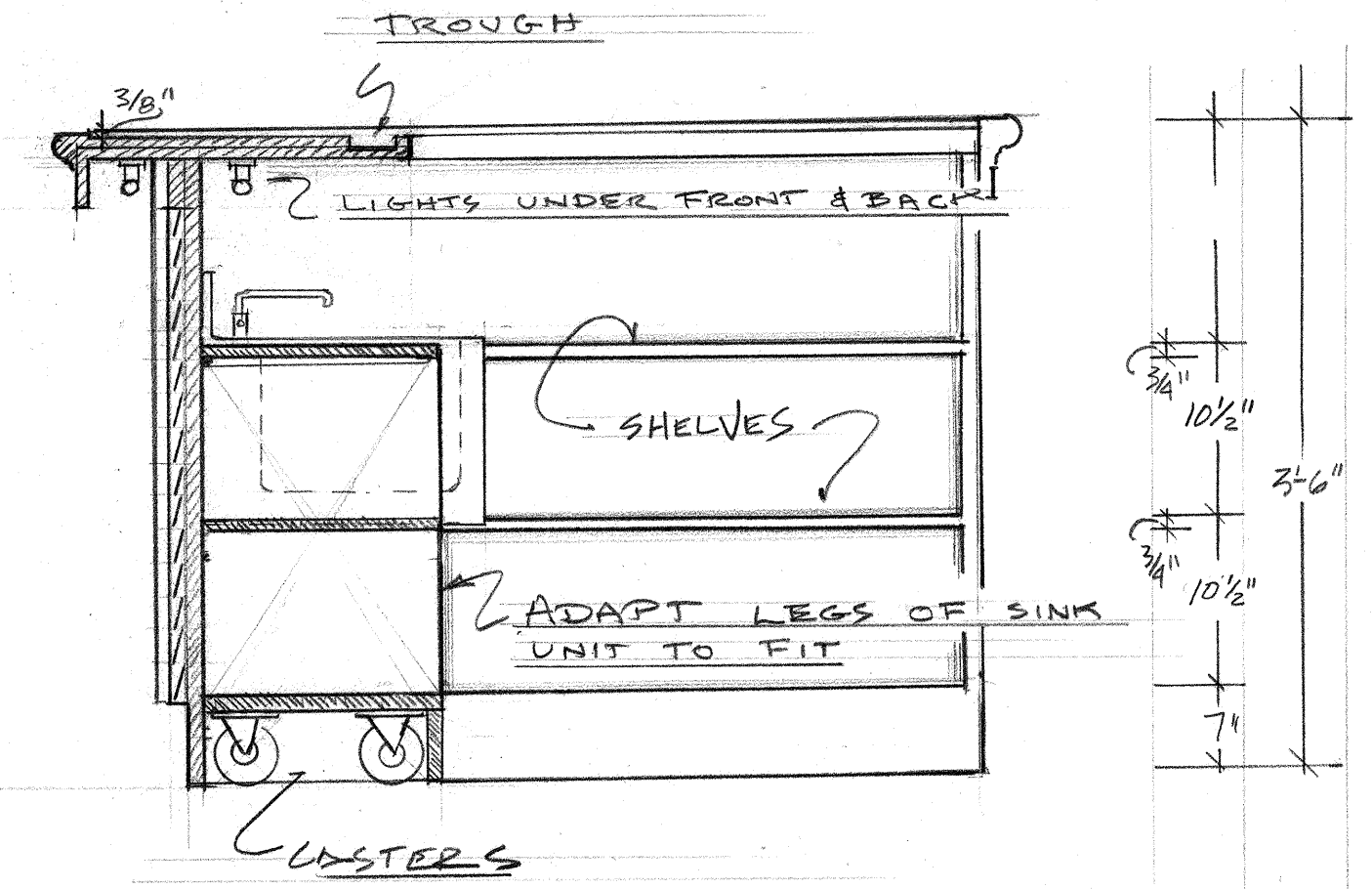
B-B. SECTION B-B SCALE 1"=1'-0"
